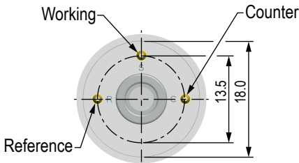
All dimensions in mm All tolerances ±0.20mm unless otherwise stated
